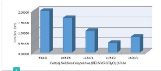
Figure 3. The pore size of PSf / PEI composite membrane prepared with variations in the composition of the coating solution
